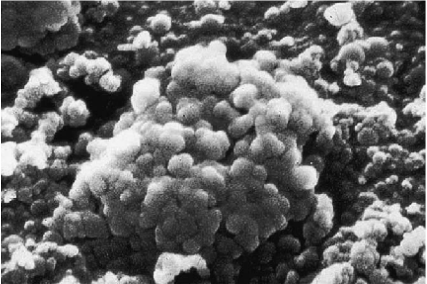
Figure 2.11 Scanning electron microscope micrograph of silica fume particles at 20,000 \times . Courtesy of Portland Cement Association.
