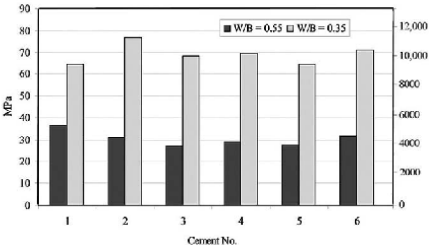
Figure 2.4 28-day compressive strength of two concretes produced at fixed water-binder ratios using six different brands of Type I cement. Note that the relative strength performance of cements that perform well in conventional-strength concrete produced at a 0.55 W/B ratio did not perform as good in high-strength concrete produced at a 0.35 W/B ratio, and vice versa. The mixtures examined contained no supplementary cementing materials or chemical admixtures.
