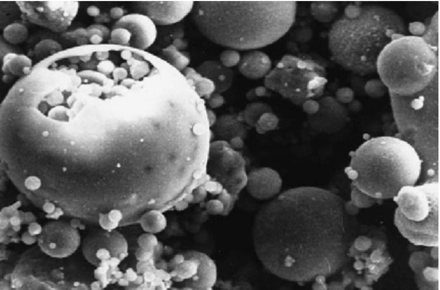
Figure 2.5 A micrograph of fly ash showing typical spherical particles. Field of view is 80 \mu\text{m} wide. Courtesy of Portland Cement Association.
