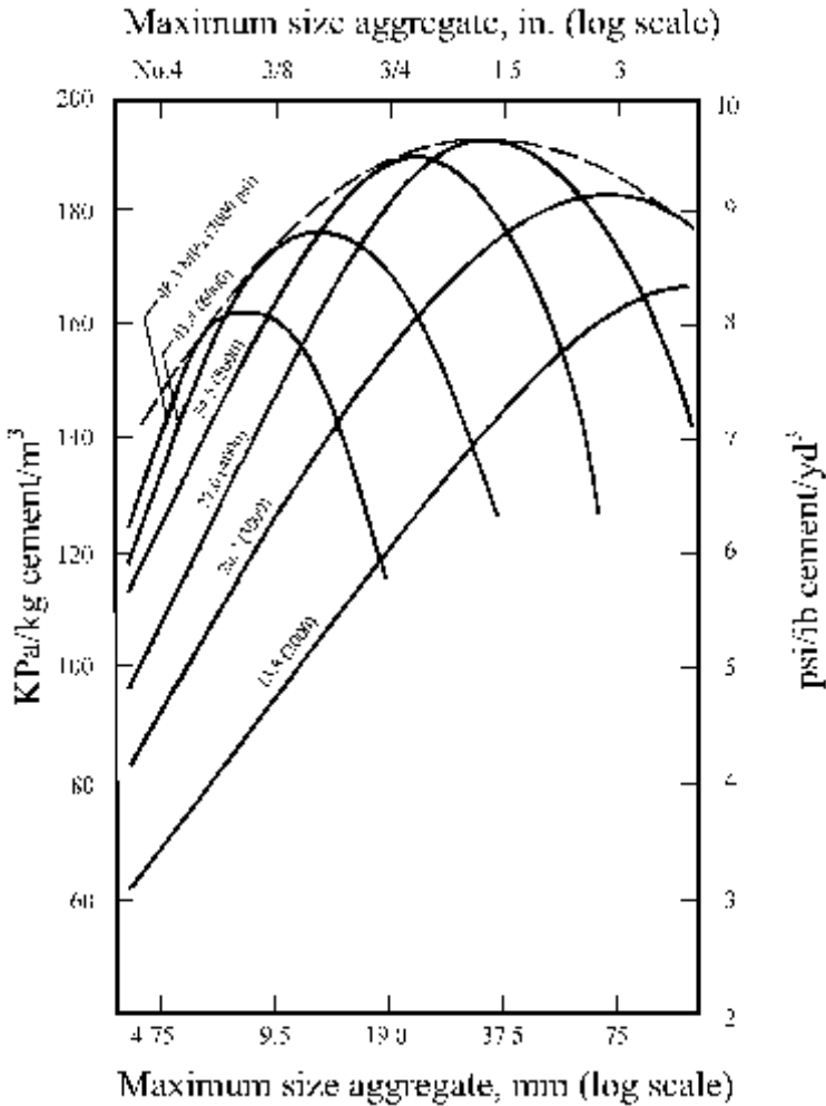
Figure 3.5 Strength efficiency of Portland cement in concretes produced with various sizes of coarse aggregates (after Farny and Panarese, 1994).
