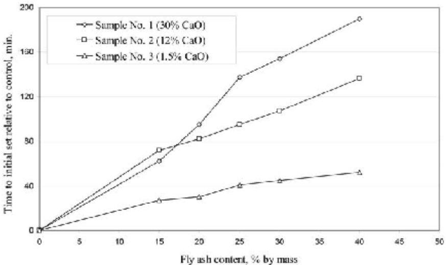
Figure 2.7 Common setting characteristics comparing low and high calcium fly ashes. Actual curves will depend on the specific fly ash used and testing conditions.
