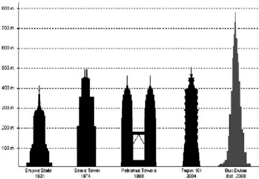
Figure 1.6 With the aid of high-strength concrete, Burj Dubai represents an extraordinary increase in attainable building height. When determining building height, spires are included whereas antennas are not.
