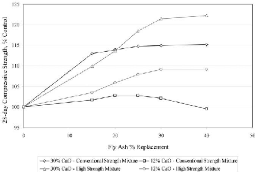
Figure 2.6 Compressive strength of concretes produced with fly ash containing 12 percent and 30 percent calcium oxide in conventional-strength and moderately high-strength concrete. The total binder content of the conventional and high-strength mixtures were 250 \text{ kg/m}^3 ( 420 \text{ lb/yd}^3 ) and 385 \text{ kg/m}^3 ( 650 \text{ lb/yd}^3 ), respectively. All batches were produced at a target slump of 125 mm (5 in).
