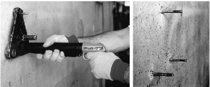
Figure 9.7 Evaluating surface hardness by means of penetration resistance method (left). Three hardened alloy-steel pins of specified hardness are driven into the surface (right). The average exposed pin length is determined by placing a triangular base plate over the pins. Courtesy of Portland Cement Association.
