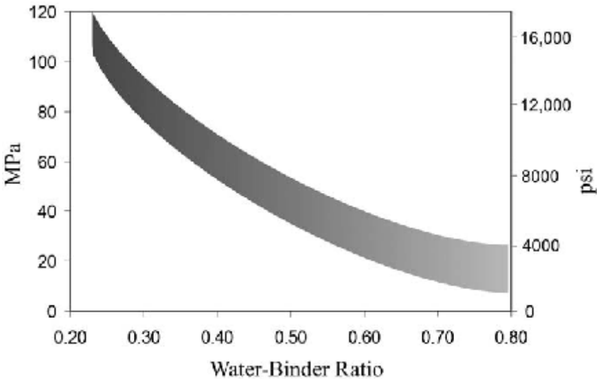
Figure 3.1 Illustration of the relationship between W/B ratio and strength for various combinations of cements and pozzolans.
