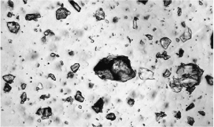
Figure 2.1 Micrograph of Type I Portland cement. Field of view is 400 \mu\text{m} wide. Courtesy of Portland Cement Association.
