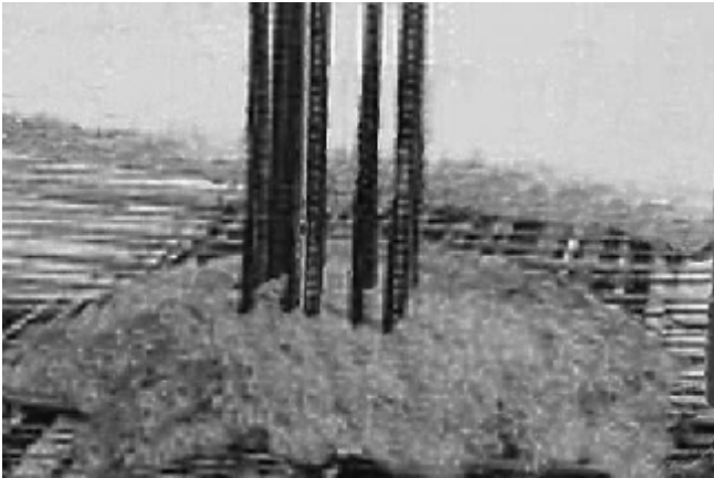
Figure 7.1 Placement of high-strength concrete simultaneously with conventional-strength concrete requires careful planning and coordination. Courtesy of CTLGroup.
