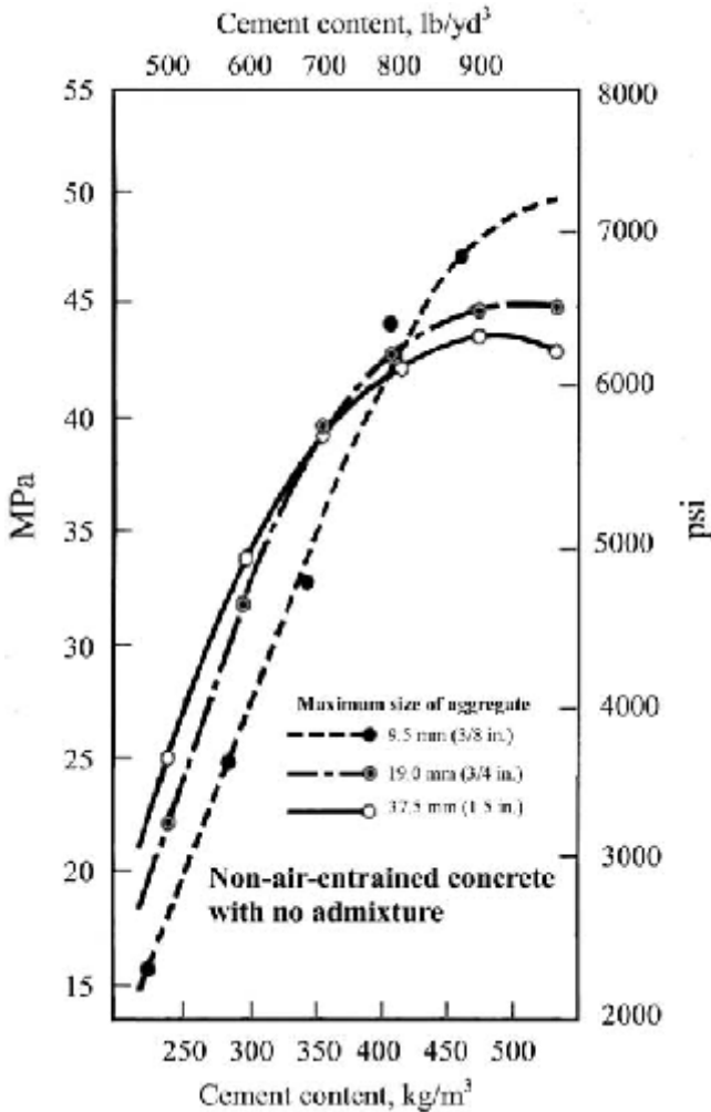
Figure 3.4 Effect of cement content on compressive strength at 28 days for various maximum sizes of aggregate (after Farny and Panarese, 1994).
