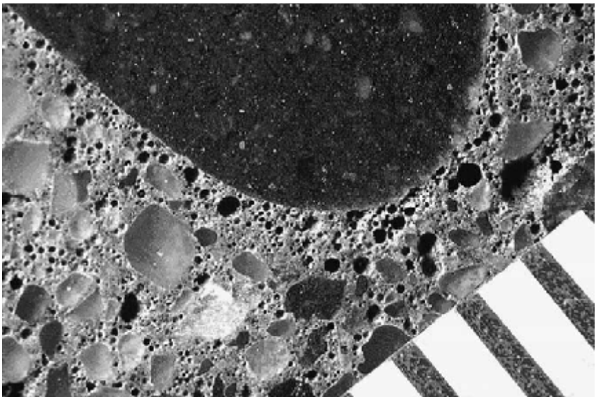
Figure 10.9 Air voids cluster along the periphery of a coarse aggregate particle. Scale in bottom right is in millimeters. Courtesy of Portland Cement Association.
