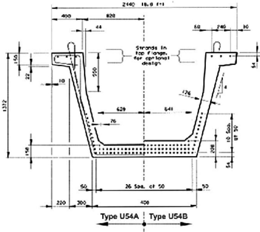
Figure 1.3 Cross section and prestressed strand patterns Texas U54 beams (after Ralls and Carrasquillo, 1994).
