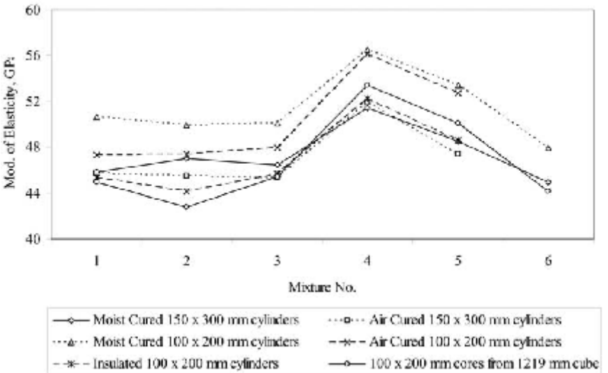
Figure 4.4 Measured modulus of elasticity at 91 days from Burg and Ost (1992) for various size cylindrical specimens cured under varying conditions.
