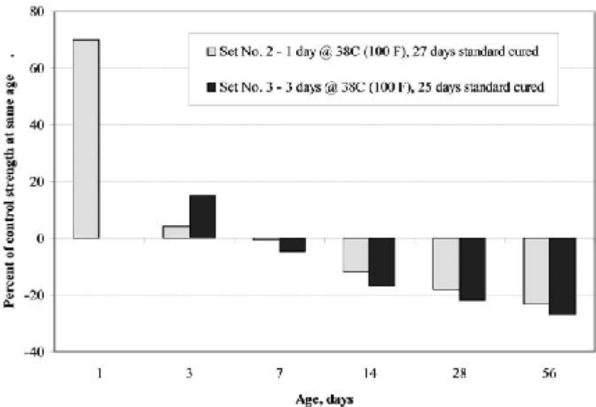
Figure 9.1 Effect of high temperature initial curing on compressive strength of 150 × 300 mm (6 × 12 in) cylinders.
