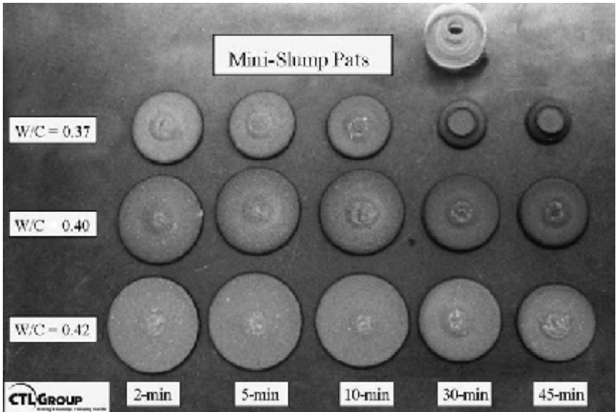
Figure 10.7 Mini-slump pats taken at 2, 5, 10, 30, and 45 minutes for mixtures produced with W/B values of 0.37, 0.40, and 0.42. Note the rapid reduction in size in the top row (W/B = 0.37), indicating rapid stiffening. Less stiffening is noted in the mixtures made with the same materials at higher W/CM values. Courtesy of CTLGroup.
