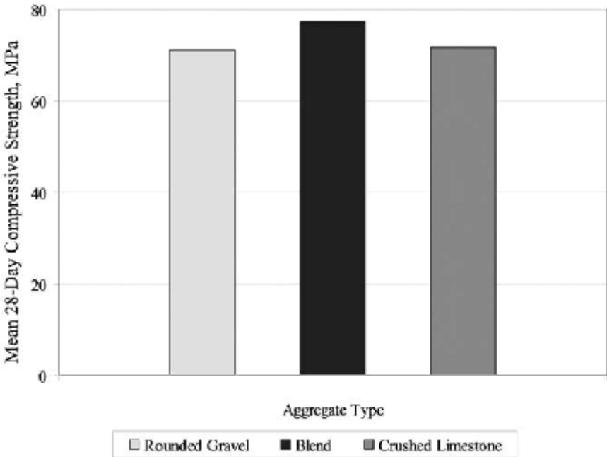
Figure 2.14 Effect of aggregate type and blend on mean 28-day compressive strength (after Luciano et al. , 1991).
