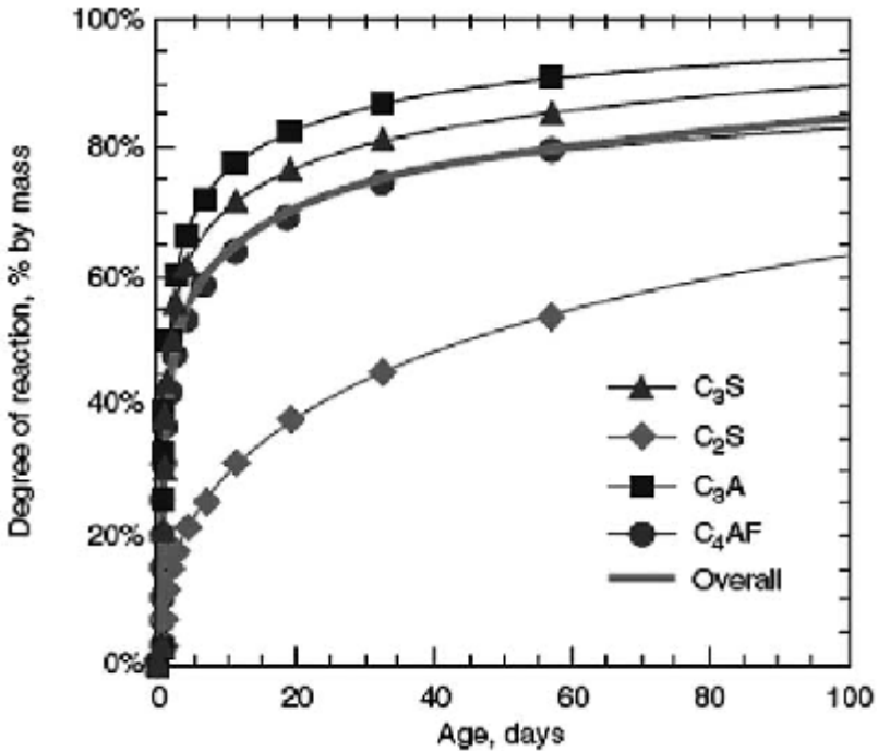
Figure 2.3 Relative reactivity of cement compounds. The curve labeled “overall” has a composition of 55 percent C 3 S, 18 percent C 2 S, 10 percent C 3 A, and 8 percent C 4 AF, an average Type I cement composition (after Tennis and Jennings, 2000).
