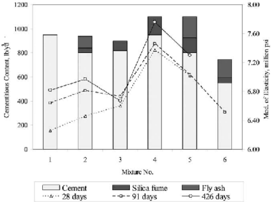
Figure 4.3b (inch-pound units) Measured modulus of elasticity at 28, 91, and 426 days from Burg and Ost (1992) for moist cured 6 × 12 in cylinders.
