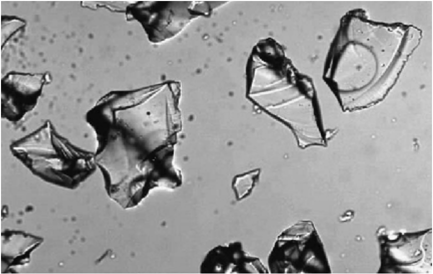
Figure 2.10 Micrograph of ground granulated blast-furnace slag grains. Field of view is 400 \mu\text{m} wide. Courtesy of Portland Cement Association.
