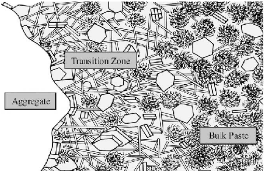
Figure 3.3 Illustration of interfacial transition zone. Courtesy of Portland Cement Association.
