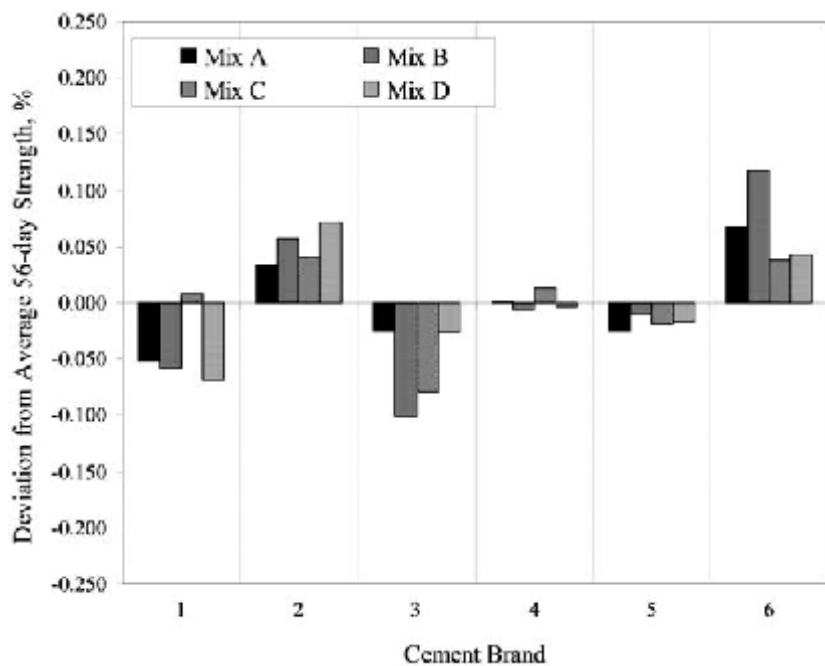
Figure 9.11 Deviation from average strength at 56 days.
