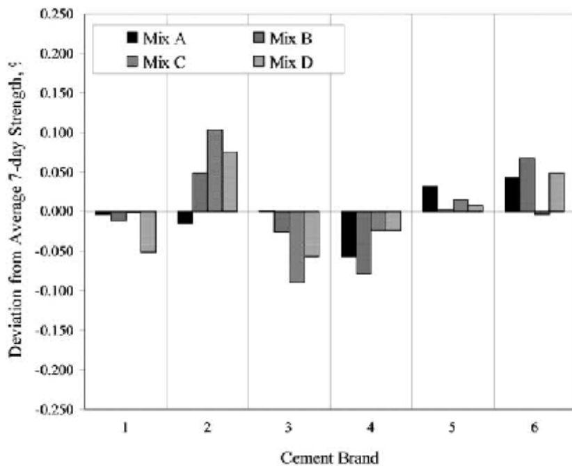
Figure 9.9 Deviation from average strength at 7 days.
