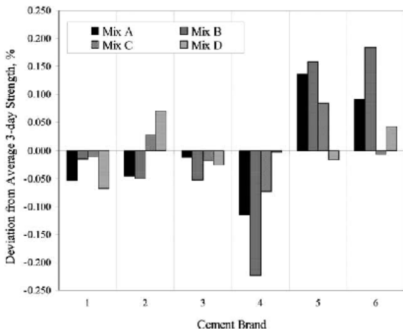
Figure 9.8 Deviation from average strength at 3 days.
