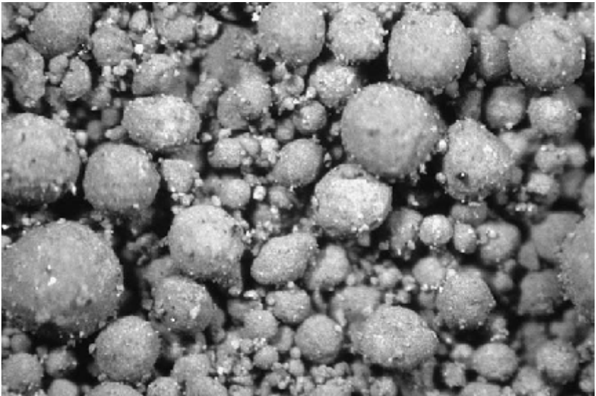
Figure 2.12 Micrograph of densified silica fume. The visible particles are agglomerations of the very small silica fume spheres, some of which can be observed adhering to the larger particles. Field of view is 200 \mu\text{m} wide. Courtesy of Portland Cement Association.
