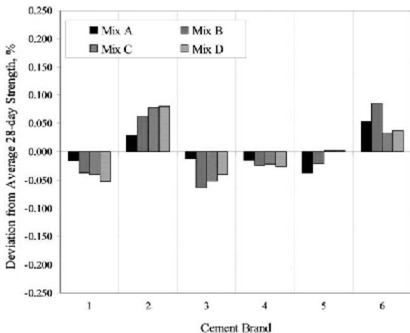
Figure 9.10 Deviation from average strength at 28 days.
