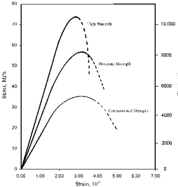
Figure 4.1 Typical stress–strain relationship for high-, moderate-, and conventional-strength concrete.
