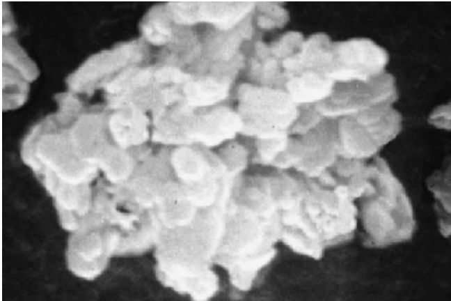
Figure 2.13 Scanning electron microscope micrograph of metakaolin particles at 20,000 \times . Courtesy of CTLGroup.
