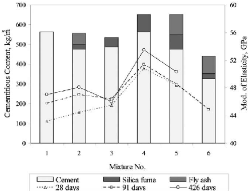
Figure 4.3a (SI units) Measured modulus of elasticity at 28, 91, and 426 days from Burg and Ost (1992) for moist cured 150 × 300 mm cylinders.
