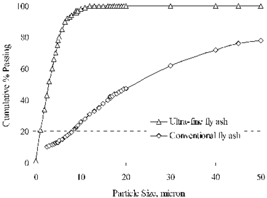
Figure 2.8 Particle size comparison of conventional and ultra-fine fly ash. Courtesy of Boral Material Technologies, Inc.
