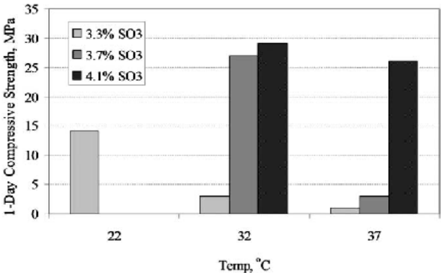
Figure 10.5 Data extracted from Cost (2006) showing 1-day strength values for mortars made using cement with various levels of sulfate, Class C fly ash used as a 25 percent cement replacement, and a carbohydrate-based water-reducing admixture. In addition to the odd behavior of decreased strength with increases in temperature, the data show the beneficial effect of additional sulfate. In this case, although the 4.1 percent sulphate resolved the strength issue, the cement was not able to pass the required ASTM C 1038 test for dimensional stability. Thus, at high temperature, the system of this cement, Class C fly ash, and this admixture placed a demand for sulfate that the cement could not supply without exceeding specification limits (after Roberts and Taylor, 2007).
