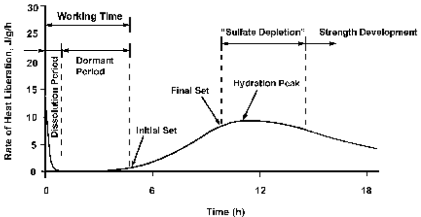
Figure 10.1 Profile of normal paste hydration.
